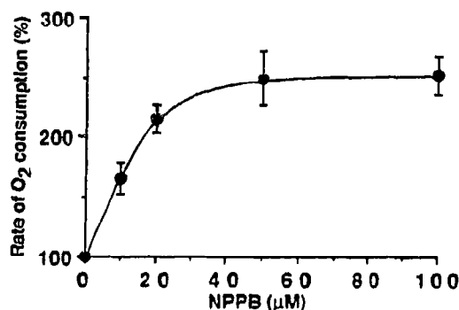
Fig. 2. NPPB stimulates O 2 consumption in macrophages in a dose-dependent manner. The experimental protocol was as in Fig. 1b. The rate of O 2 consumption is expressed as percent of the resting level. Data are means of 3–5 experiments \pm SE.
