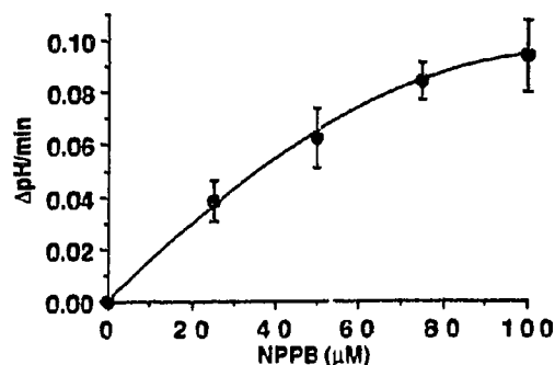
Fig. 4. The rate of conductive proton transport across the plasma membrane of human neutrophils as a function of NPPB concentration. Proton movements were determined in K^+ medium in the presence of the indicated concentration of NPPB as described in Fig. 3b. Data are means of at least 3 experiments \pm SE.
