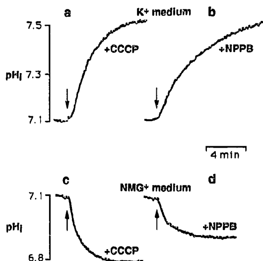
Fig. 3. NPPB and CCCP increase the plasma membrane proton permeability in human neutrophils. Cytosolic pH ( pH_i ) changes were measured using the fluorescent indicator BCECF. BCECF-loaded neutrophils ( 10^6/ml ) were suspended in K^+ medium (140 mM KCl, mM CaCl_2 , 1 mM MgCl_2 , 10 mM glucose, 20 mM HEPES, pH 7.7; panels a and b) or NMG^+ medium (140 mM NMG-Cl , 3 mM KCl, 1 mM CaCl_2 , 1 mM MgCl_2 , 10 mM glucose, 20 mM HEPES, pH 7.7; panels c and d) at 37^\circ C in the presence of 1 \mu M CCCP (a and c) or 100 \mu M NPPB (b and d). After a steady-state pH_i was attained, conductive proton movements were induced by increasing the plasma membrane K^+ permeability with 1 \mu M valinomycin (arrows). Representative of 3-4 experiments.
