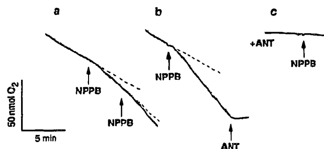
Fig. 1. NPPB stimulates mitochondrial oxygen consumption in macrophages. Macrophages ( 2 \times 10^6 /ml) were suspended in Na + medium and O 2 consumption was measured with a Clark electrode. Additions: a, NPPB 10 \mu M; b, NPPB 100 \mu M, antimycin A (ANT) 5 \mu g/ml; c, antimycin A 5 \mu g/ml was present in the medium prior to addition of cells, NPPB 100 \mu M added where indicated. Traces are representative of 3–5 experiments.
